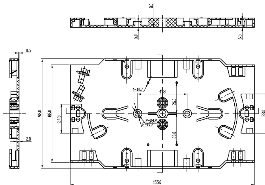
Dimensional drawing
