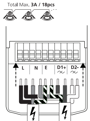
4d 220-240V~ + DALI Total Max. 3A / 18pcs
