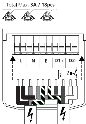
4b 220-240V~ + Switch-Dim Total Max. 3A / 18pcs
