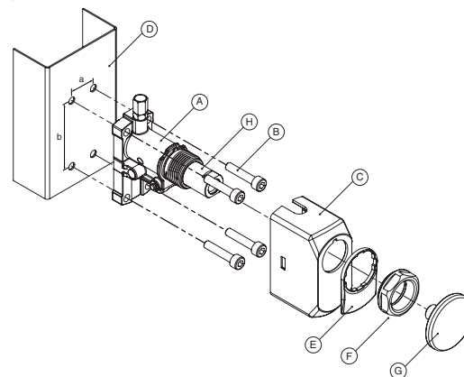
Fixing to the outside of the profile
