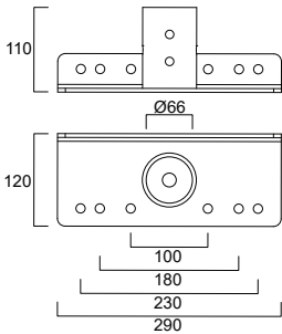
Raiden Post Top Adaptor 60mm
