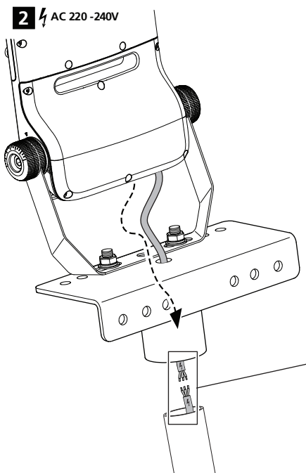
Raiden Post Top Adaptor 60mm
