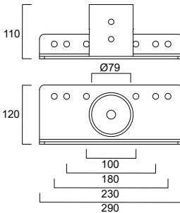
Raiden Post Top Adaptor 76mm
