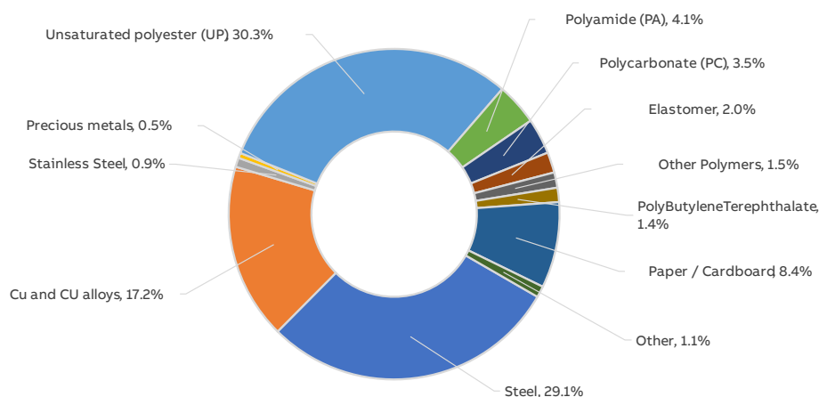
Figure 1: Composition of XT2 160 N/S/H/L/V 3P IEC Ekip
