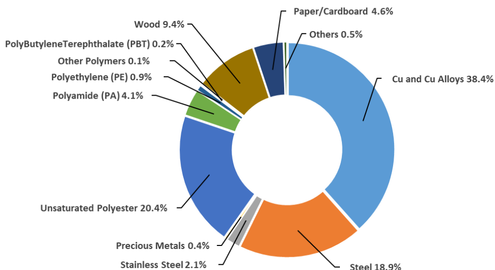
Figure 1: Composition of AF2650-30-11
