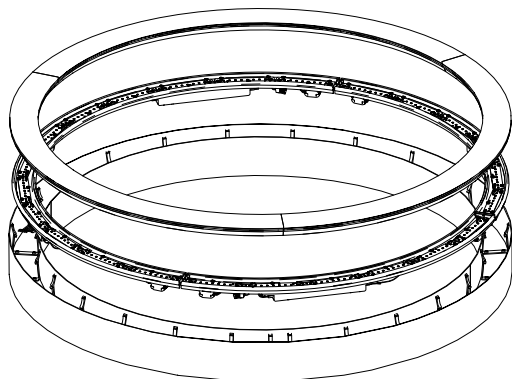
2x180°/1174, 4x90°/1530 LED-Lichteinsatz | LED light insert | Insert lumineux LED | Inserto luminoso a LED
