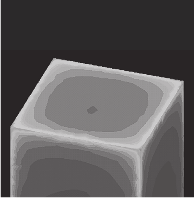
Figure 3. Electric field plot of a real structure in an ambient field, showing that the intensification is high at the corners, moderate on the horizontal and upper vertical edges and very low on flat horizontal and vertical surfaces.
