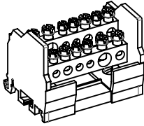
BD Two Pole Distribution Block, 80/100AL BD-80-100AL (563910)
