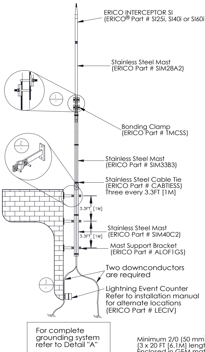
Mast Detail
