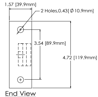
② Typical ALOF1GS Wall Bracket Base Not to Scale
