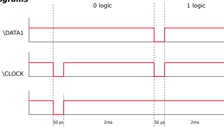
Open collector output with internal pulls up 1K at +5V or +12V according the ST4 position.
