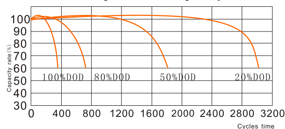
Cycle life curves (25°C) / Courbes de cycle de vie (25°C)
