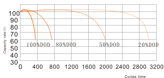
Cycle life curves (25°C) / Courbes de cycle de vie (25°C)
