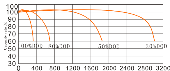
Cycle life curves (25°C) / Courbes de cycle de vie (25°C) Discharge at 0.1C / Cut off voltage 1.8V by cell
