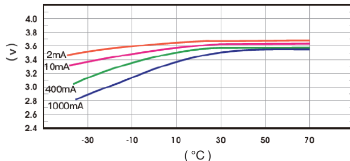
Characteristics of voltage platform at different temperatures
