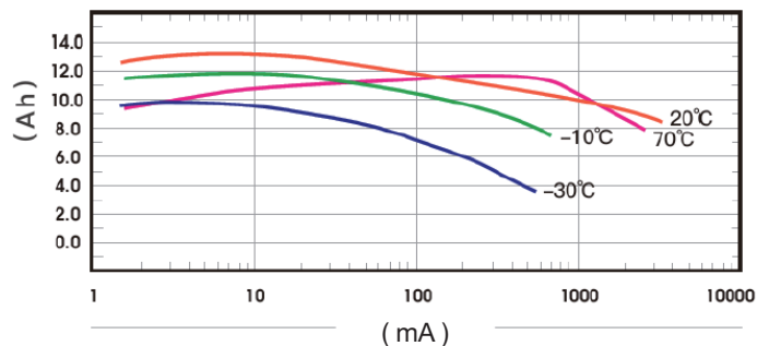
Different discharge current and discharge capacity characteristics
