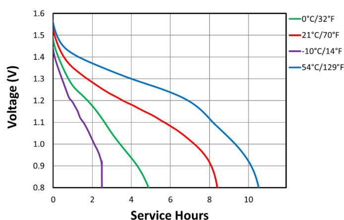
Constant Current - 250 mA
