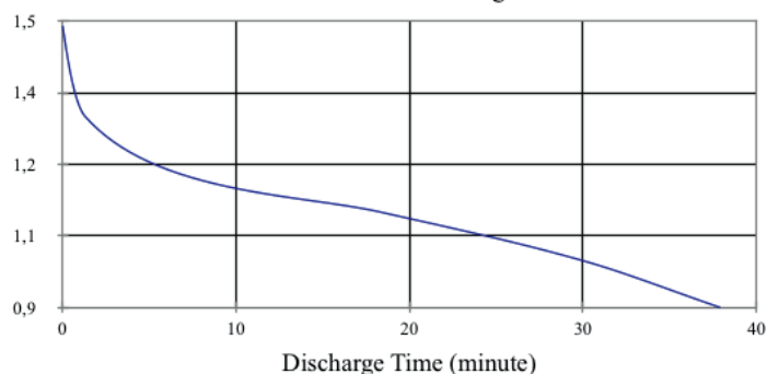
3.9Ω Continuous Discharge Curve
