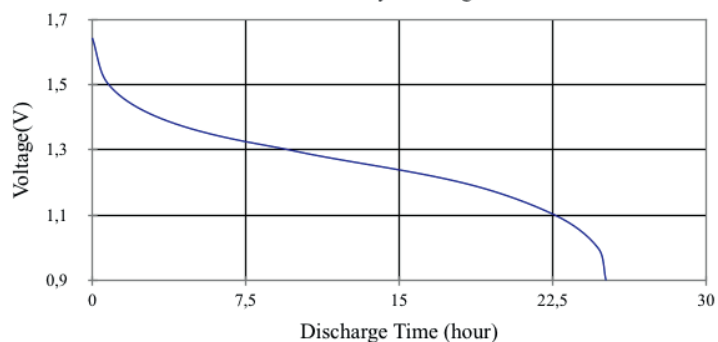
75Ω 4hour/day Discharge Curve
