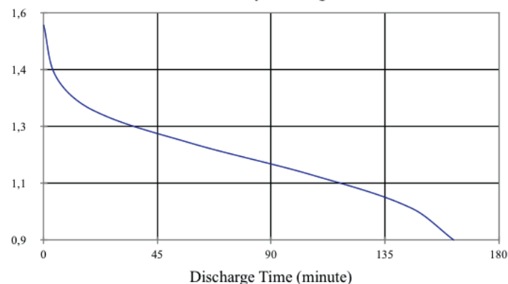
10Ω 1hour/day Discharge Curve
