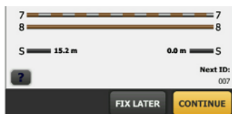
Wiremap – shows distance to fault, break and short
