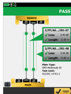
Complete data is displayed with a test result. The dotted line shows what's included in the measurement. Detail windows show the results for each fiber tested.
