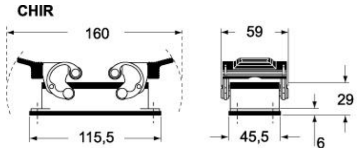
Catalogue drawings
