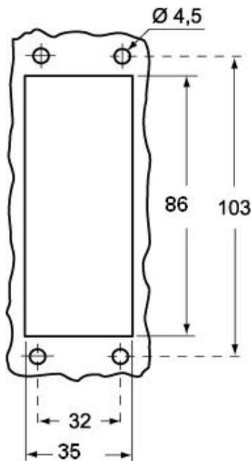
Catalogue drawings
