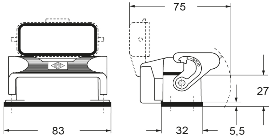
Catalogue drawings
