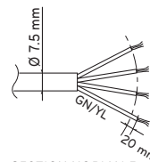
SECTION NORMALE DU TUYAU 0.75 mm 2 H07RN-F
