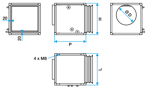
Dimensions Batteries
