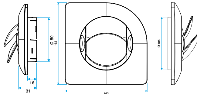
Grille BIO Design carré D 125 mm
