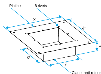
Clapet anti-retour VELONE
