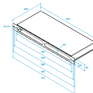
Encombrement MEA 200
