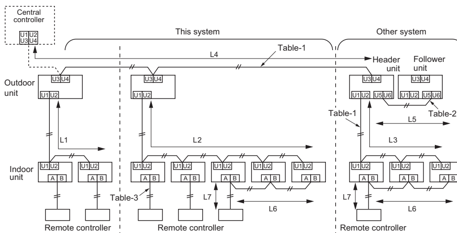
Wiring 2-core, non-polarity Type Shield wire Size/Length*1 1.25 mm 2 : Up to 1000 m 2.0 mm 2 : Up to 2000 m
