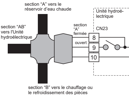
▼ Fig.7-26 Type 3 SPDT
