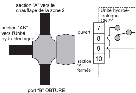
▼ Fig.7-28 Type 2 SPST
