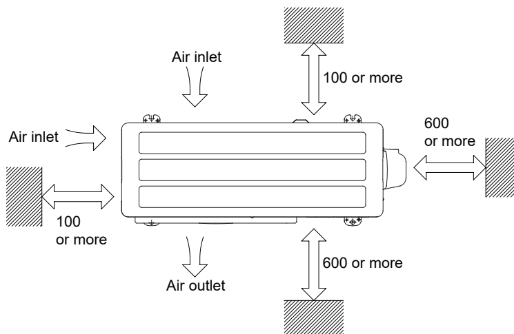
Installation dimension
