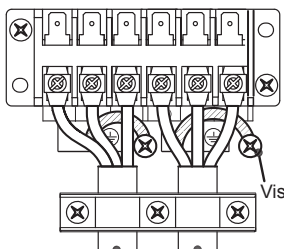
Câble de raccordement (Unité C) Câble de raccordement (Unité D)
