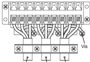
Câble de raccordement (Unité C) Câble de raccordement (Unité D)
