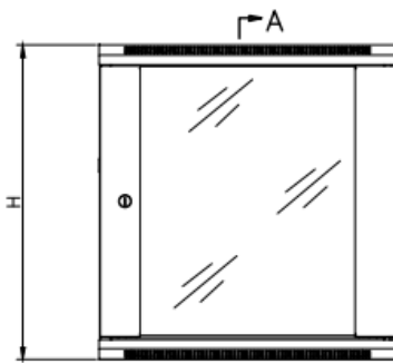
front door(glass)
