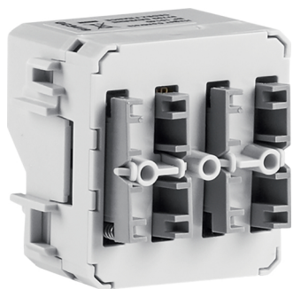
WNT331
