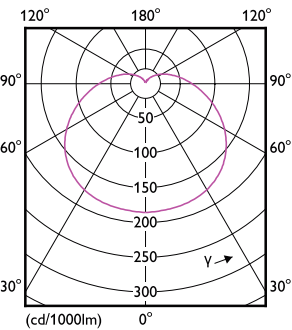
LEDbulb 15 5-120W A67 E27
