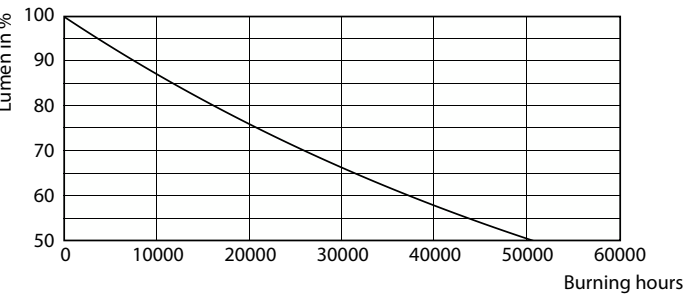
Lumen Maintenance Diagram - MAS LEDCandleDT5.9-60W E14 927 B35 CL G
