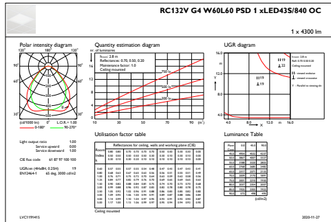
IFGU1_RC132VG4W60L60PSD1xLED43S840OC
