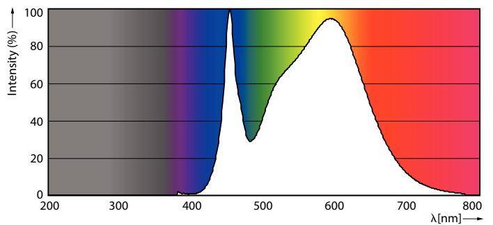
Spectral Power Distribution Colour - MAS LEDtube 1500mm HO 26W 840 T5
