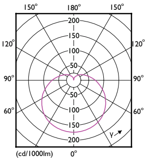
Light Distribution Diagram - CorePro LEDbulb ND 13-100W A60 E27 930
