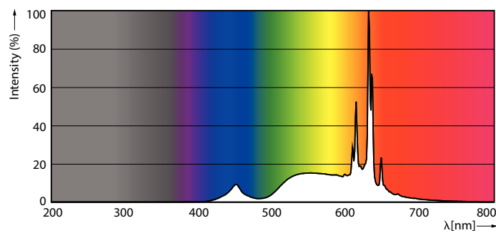
Spectral Power Distribution Colour - MAS VLE LEDBulbDT5.9-60W E27 927A60CL G
