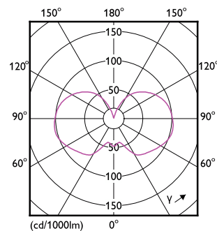
Light Distribution Diagram - MAS VLE LEDBulbDT5.9-60W E27 927A60CL G
