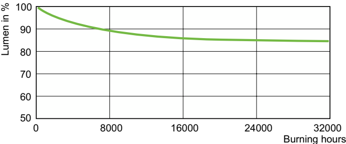
Lumen Maintenance Diagram - MASTER GreenPower 600W 400V E40
