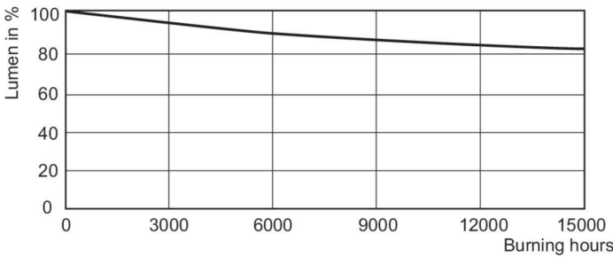
Lumen Maintenance Diagram - MASTER SDW-T 35W/825 PG12-1 1SL/12
