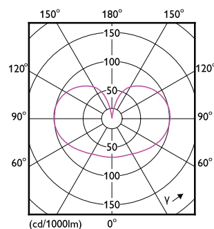
Light Distribution Diagram - CorePro LEDBulbND 120W E27 A67 840 CL G
