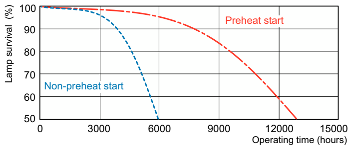
Life Expectancy Diagram - PL-Q 38W/840/4P 1CT/10BOX
