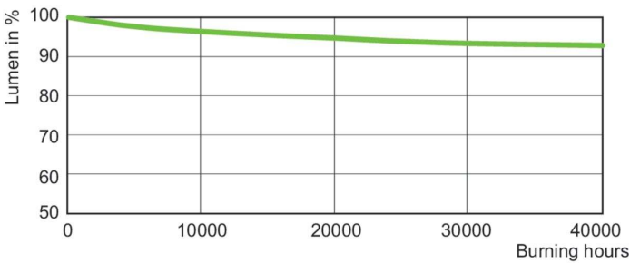
Lumen Maintenance Diagram - MST SON-T APIA Plus Xtra 250W E40 1SL/12
