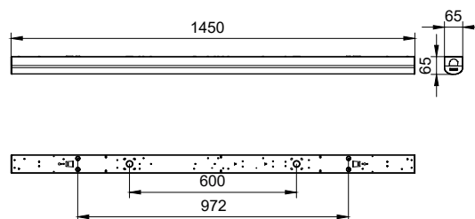
BN126C LED74S/830 PSU TW1 L1500
