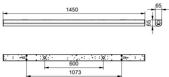
BN126C LED74S/830 PSU TW1 L1500
