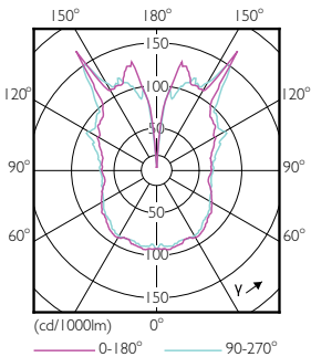
LEDbulb Class-giant 40W E27 G200 Gold DIM
