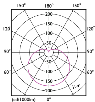
Light Distribution Diagram - LEDbulb ND 10-75W A60 E27 827 6CT
