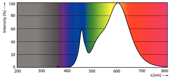
Spectral Power Distribution Colour - TForce Core HB MV ND 30W E27 830 G3
