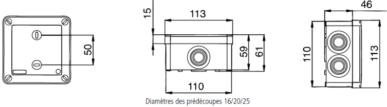
Pico BDD-FLD 100x100
