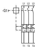
Figure 2: Circuit diagram of the PKZM0-.../XTPR...BC1NL, PKZM0-...-T/XTPPT...BC1NL motor-protective circuit-breakers
