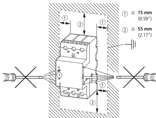
Figure 6: Mounting the PKZM0-.../XTPR...BC1NL and PKZM0-...-T/XTPT...BC1NL
