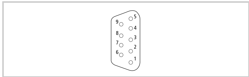
Fig.. 24 Profibus interface (9-pin, D-Sub, female, UNC)
